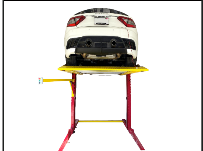
CLEARANCE BETWEEN COLUMNS 82 3/4" (2100MM) RAISED HEIGHT 82 3/4" (2100MM) FOR CARS & SUV'S
