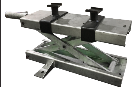
MECHANICAL JACK
