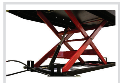
HEAVY DUTY SCISSOR DESIGN PROVIDES BETTER STABILITY WHEN LIFTING HEAVIER EQUIPMENT.
